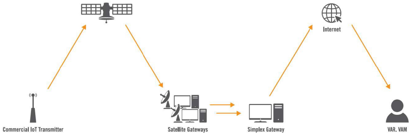
FIGURE - IoT MESSAGING
