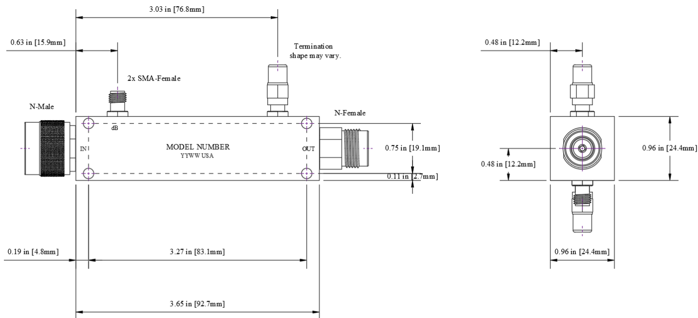
Outline drawing # OL-AIRCPL-1030-1 (Werbel reference).
