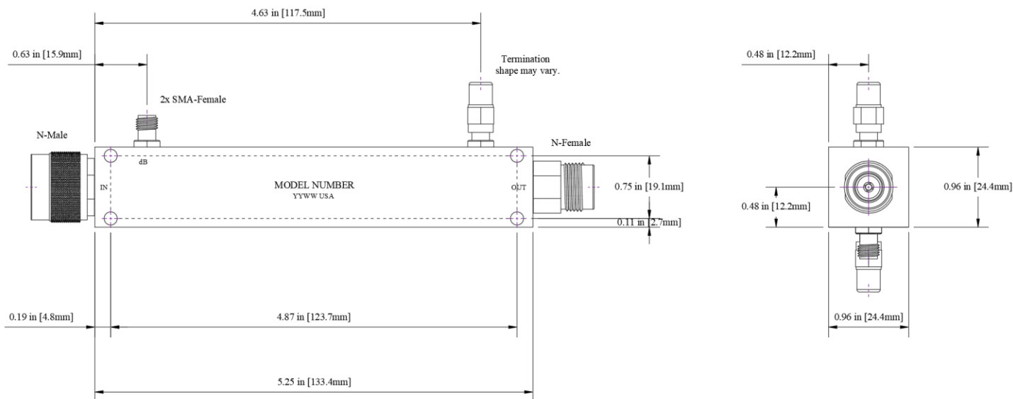
Outline drawing # OL-AIRCPL-0510-1 (Werbel reference).
