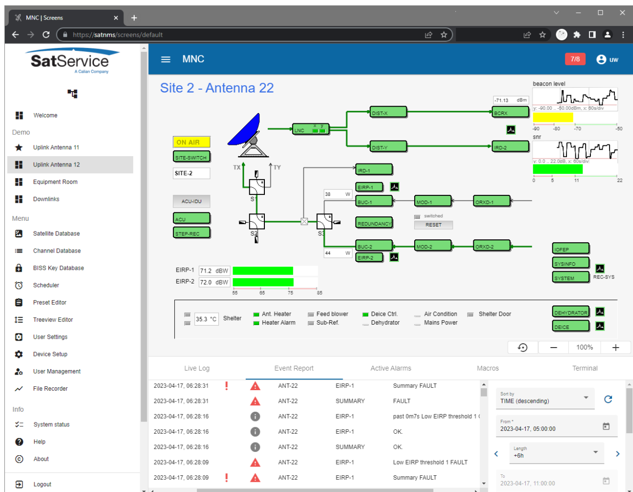
Figure 1: Typical web interface for uplink station
