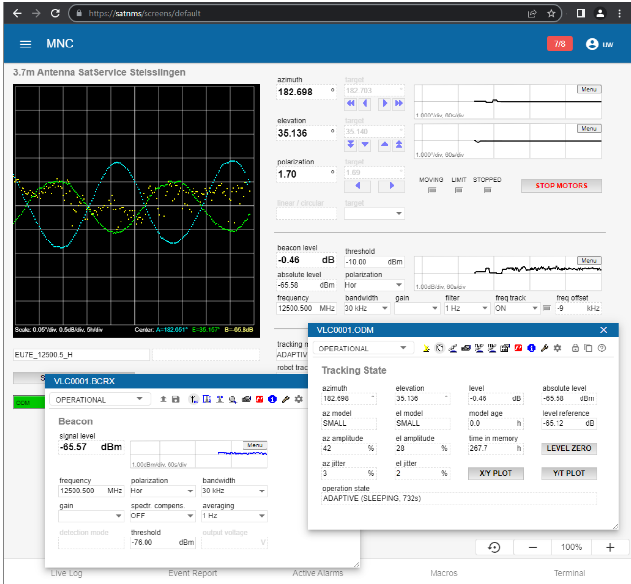
Figure 5: comprehensive screen for an antenna tracking system and ACU and beacon receiver device windows
