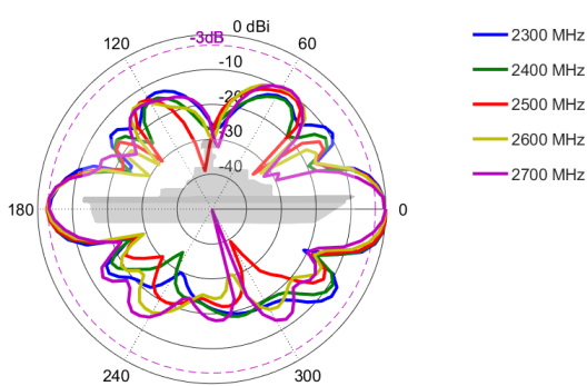
Elevation: 2300 – 2700 MHz
