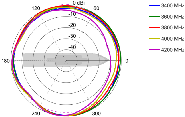
Azimuth: 3400 – 4200 MHz
