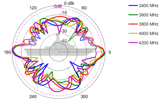
Elevation: 3400 – 4200 MHz
