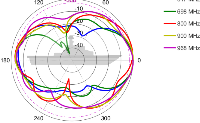
Elevation: 617 – 968 MHz
