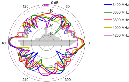
Elevation: 3400 – 4200 MHz
