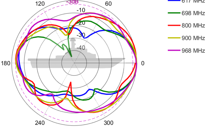
Elevation: 617 – 968 MHz
