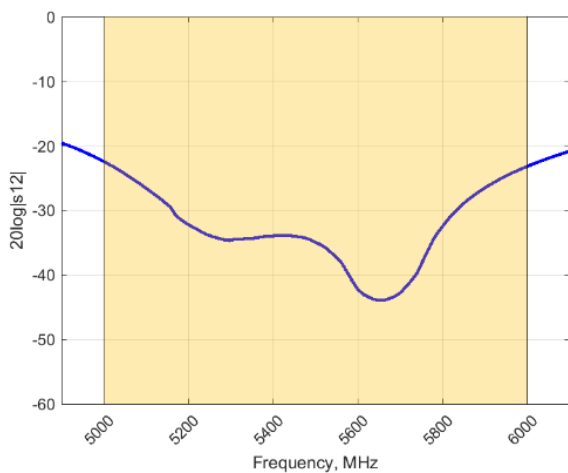
Isolation: 5000 – 6000 MHz
