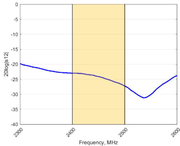
Isolation: 2400 – 2500 MHz
