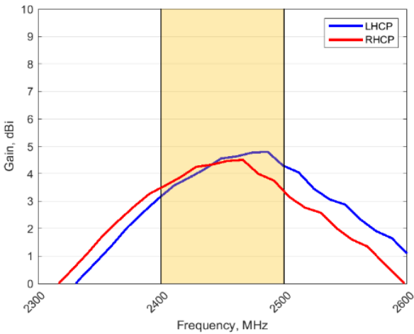
GAIN (EXCLUDING CABLE LOSS): 2400 – 2500 MHz
