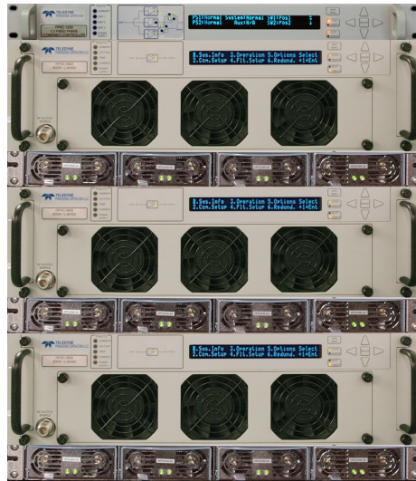
300W C-Band, 1:2 3RU Phase Combined System with FPRC-1200 Controller
