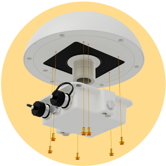
Ethernet Splitter
