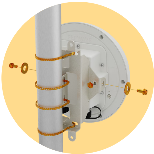
Pole Mounting
