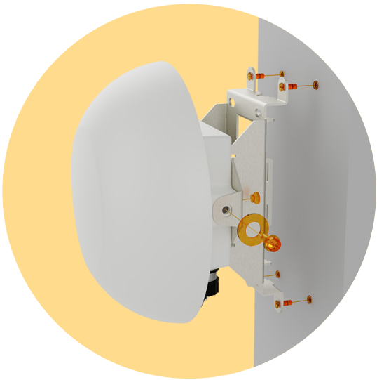
Wall Mounting
