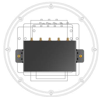
5G Adapter
