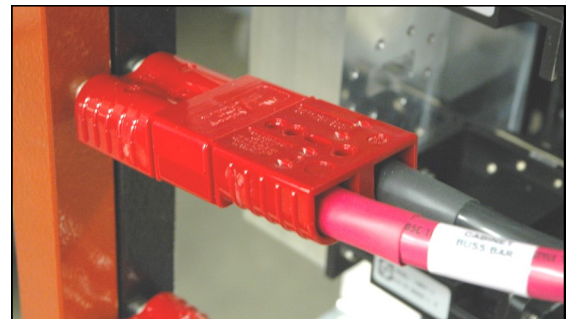
Quick Connect Plug into Bus Rail
