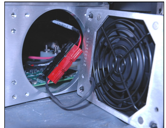
Removable rear panel fan tray
