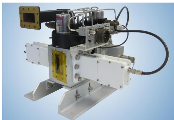
Typical C-Band 1:2 LNB Plate Assembly
