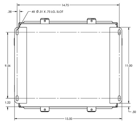
MOUNTING DETAILS
