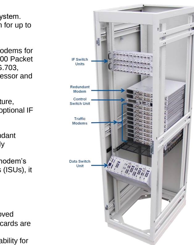
CRS-500 1:N Modem Redundancy System Typical Rack View (back side)
