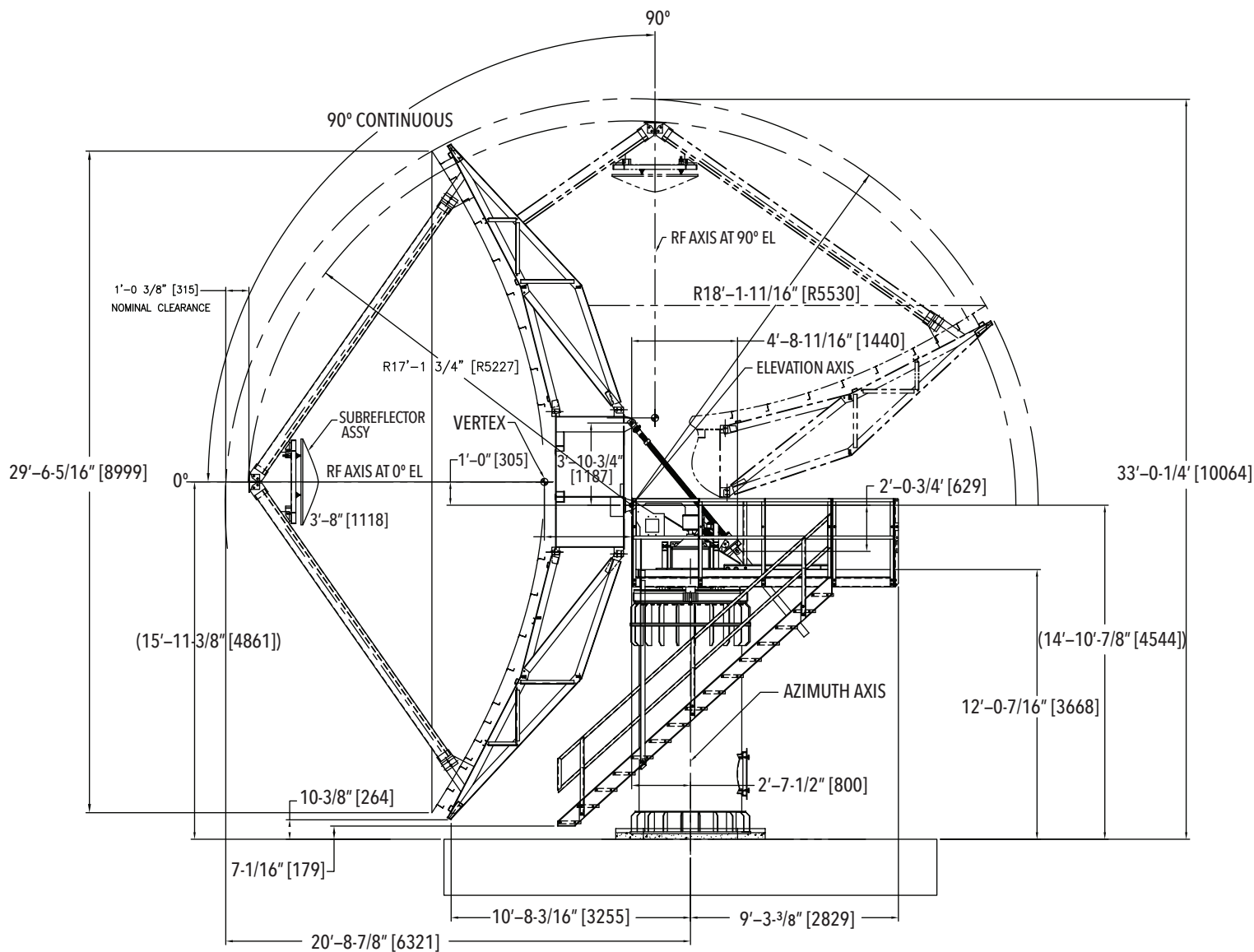
ELEVATION VIEW
