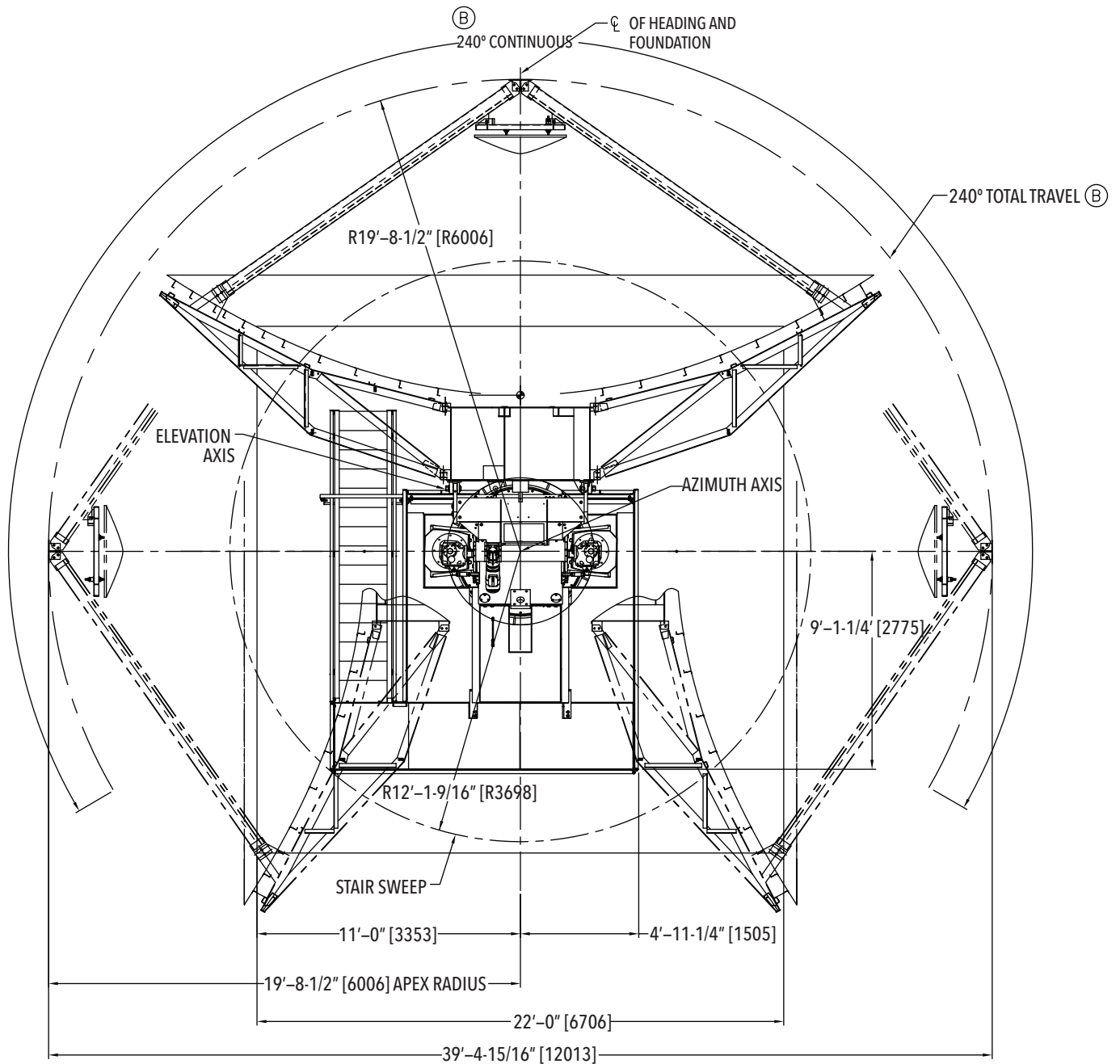
PLAN VIEW
